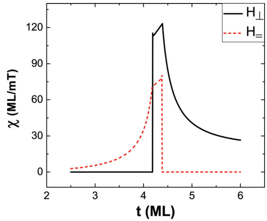
FIG. 4. (Color online) Calculated film thickness dependence of magnetic susceptibilities for Co/Au(111). The ac modulation field of 0.12 mT or 0.05 mT is oriented within ( H_{\parallel} ) or perpendicular to the sample plane ( H_{\perp} ), respectively.
