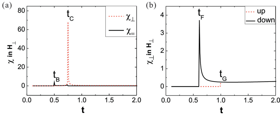
FIG. 2. (Color online) (a) Thickness dependence of the perpendicular (dashed line) and in-plane (solid line) susceptibilities around the SRT via a canted state. The ac modulation field is applied perpendicular to the sample plane. (b) The perpendicular susceptibility around the SRT via a coexistent state in perpendicular ac modulation field. Line up (dashed line) and down (solid line) represent that the magnetizations in the coexistent region orient either fully perpendicular or fully within the sample plane, respectively.
