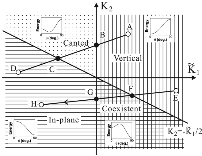
FIG. 1. The energy phase diagram in the anisotropy space. The insets show a typical angle-dependent energy of each state. Linear trajectory AD and EH represent thickness-driven SRT via a canted state and a coexistent state, respectively.
