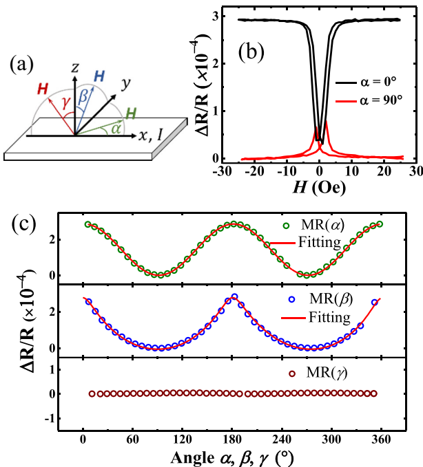
FIG. 1. (a) Spatial coordinates of the measurements, where the current is along the x -axis. (b) MR of the YIG (20 nm)/Pt (5 nm) bilayer for \alpha = 0^\circ and \alpha = 90^\circ . (c) MR as functions of the magnetic field directions with H = 3000 Oe. The red curves are fitting lines according to the SMR theory.
