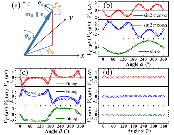
FIG. 3. (a) Spatial coordinates of the precession of \mathbf{M} , where \mathbf{m}_0 denotes the unit vector in the direction of the equilibrium magnetization. (b)–(d) \alpha , \beta , and \gamma dependence of V_A (red circles), V_S (blue circles), and V_C (green circles), respectively. The red and blue solid curves are the fittings to Eqs. (3) and (4) ( \alpha -scan) or Eqs. (5) and (6) ( \beta -scan). The green solid curves are the fittings according to the spin Seebeck effect scenario.
