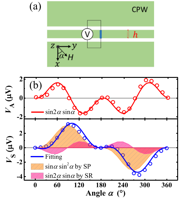
FIG. 4. (a) Sketch of the experimental set-up. A short sample was placed in the center of the CPW with \mathbf{h} mainly along the x -axis. (b) V_A (red circles) and V_S (blue circles) as a function of \alpha . The red solid curve is the fitting according to Eq. (7). The blue curve is the fitting according to Eq. (8). The dc voltage is the superposition of SPE (yellow) and SRE (pink) components.
