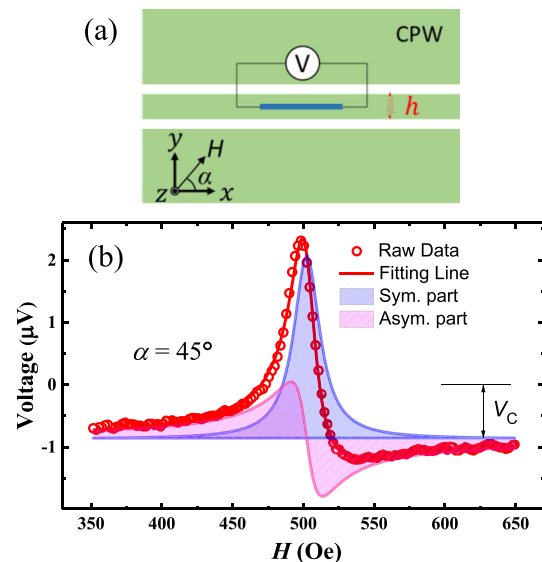
FIG. 2. (a) Sketch of the experimental set-up. The YIG/Pt bilayer was placed upside down along the signal line of the CPW with \mathbf{h} mainly along the y -axis. (b) The dc voltage (open circles) was detected by sweeping H at \alpha = 45^\circ . The red fitting line is given by a superposition of symmetric (blue) and antisymmetric (pink) components after removing a constant value V_C , originated from the spin Seebeck effect.
