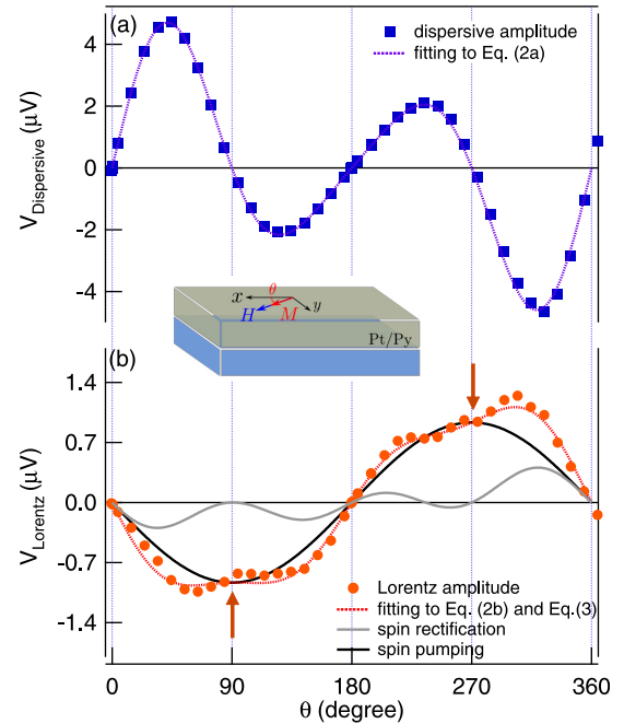
FIG. 3. At 8 GHz, the dispersive and Lorentz line shape components of the DC voltage as a function of \theta are plotted in (a) and (b), respectively. The dispersive component in (a), which is a pure spin rectification signal, is seen to cross zero when \theta equals to 0^\circ , 90^\circ , 180^\circ , and 270^\circ . The Lorentz component contains contributions from both spin rectification and spin pumping. The contribution due to spin rectification crosses zero at the same angles as (a), but the spin pumping contribution does not cross zero at \theta of 90^\circ and 270^\circ .
