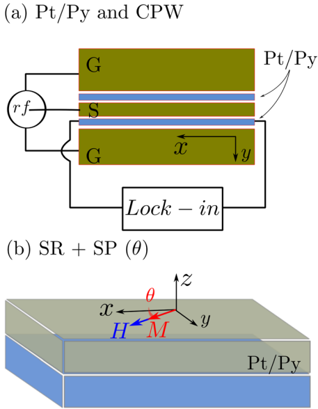
FIG. 1. (a) The Pt/Py bilayer was patterned in between the G and S lines of the CPW. (b) While the external magnetic field \mathbf{H} is applied in the x - y plane, a DC voltage due to both spin rectification and spin pumping can be detected.
