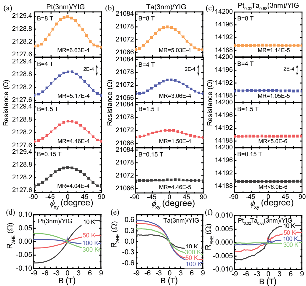
FIG. 3. Room temperature angular dependent MR as a function of \phi_{xy} for (a) Pt (3 nm)/YIG, (b) Ta (3nm)/YIG, and (c) \text{Pt}_{0.32}\text{Ta}_{0.68} (3 nm)/YIG measured at 0.15 T (black), 1.5 T (red), 4 T (blue), and 8 T (orange), respectively. (d)–(f) The temperature dependent AHE for Pt (3 nm)/YIG, Ta (3 nm)/YIG, and \text{Pt}_{0.32}\text{Ta}_{0.68} (3 nm)/YIG, respectively, is shown.
