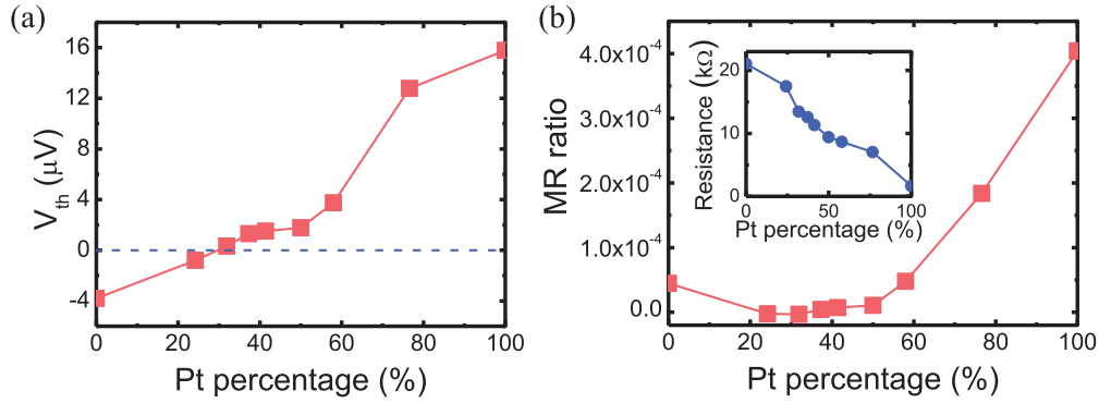
FIG. 2. (a) Thermal voltage V_{th} with perpendicular temperature gradient and (b) MR ratio for 3-nm \text{Pt}_\delta\text{Ta}_{1-\delta} alloy on YIG substrate at different Pt percentage at room temperature. The insert of (b) presents the dependence of resistance 3-nm \text{Pt}_\delta\text{Ta}_{1-\delta} alloy on Pt component.
